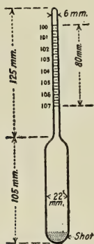
FIG. 153.—Hydrometer.
